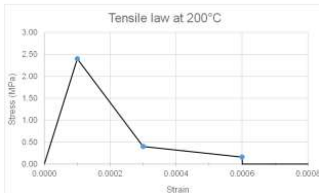
Figure 10: Tensile law at 200°C.
